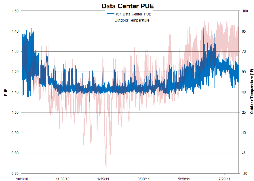
Figure 4. NREL's data center PUE.
