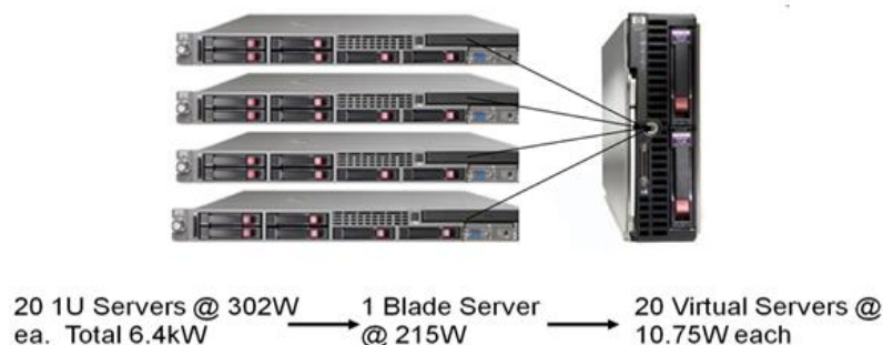
Figure 2. Data center blade server virtualization ratio. Illustration courtesy of NREL.
