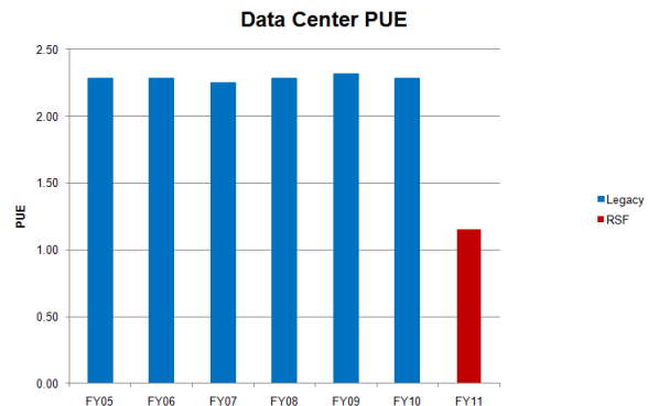
Figure 7. PUE comparison of NREL's RSF data center to the legacy data center.
